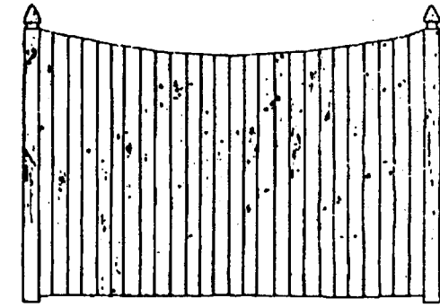
DECORATIVE BOARD SOLID SINGLE CONCAVE W303
